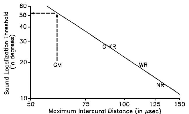
Figure 4. Relation between head size (maximum interaural distance) and sound localization threshold among rodents. (The correlation based on herbivorous [nonpredatory] rodents is 0.98 ( p < .05 ). This relation results in a predicted threshold for the grasshopper mouse of 53^\circ —far greater than its actual threshold of 19^\circ —suggesting that predatory rodents are under more selective pressure to localize sound accurately. G, gerbil; GM, grasshopper mouse; KR, kangaroo rat; NR, Norway rat; WR, wood rat. See Table 2 for references.)
