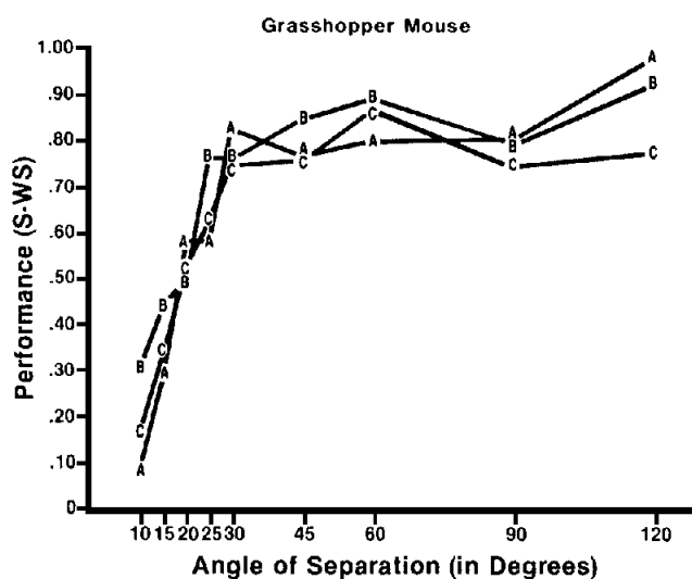
Figure 3. Sound localization performance in the azimuthal plane, calculated by the formula S - WS , for three grasshopper mice. (A, B, and C represent individual animals.)
