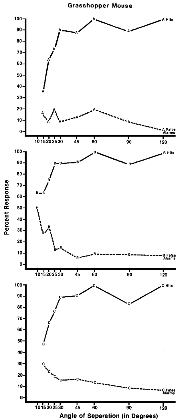
Figure 2. Percentages of hits (correct detections) and false alarms for the three grasshopper mice. (Note different false alarm rates of the three mice as threshold was approached. A, B, and C represent individual animals.)
