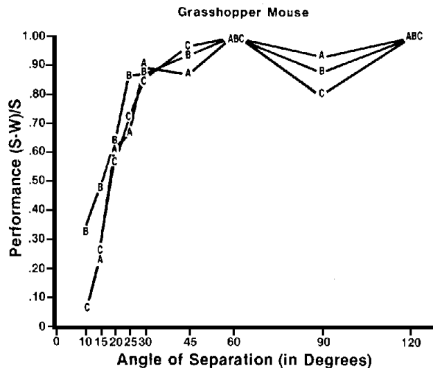
Figure 1. Sound localization performance in the azimuthal plane, calculated by the formula (S - W)/S , for three grasshopper mice. (A, B, and C represent individual animals.)
