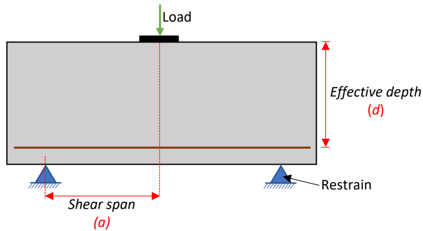
Figure 2-5: Shear span to depth ratio of a typical deep foundation.
