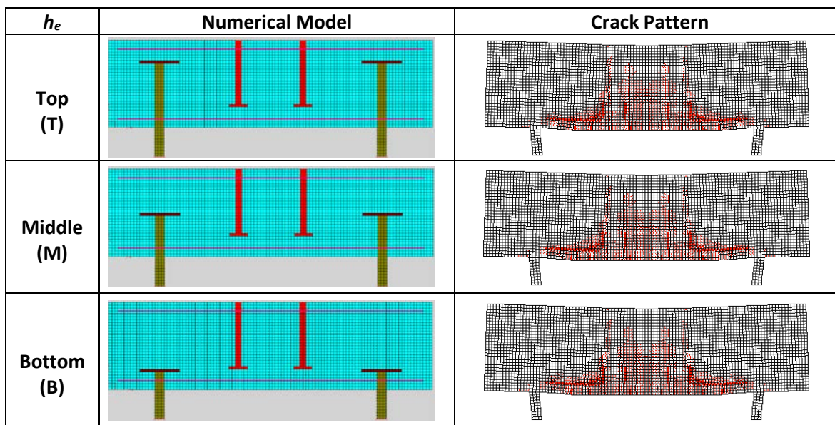
Figure A-27: Numerical model and crack pattern-single bracket type-monotonic compression - a/d ratio = 1.42, \rho_x = 0.4\% .
