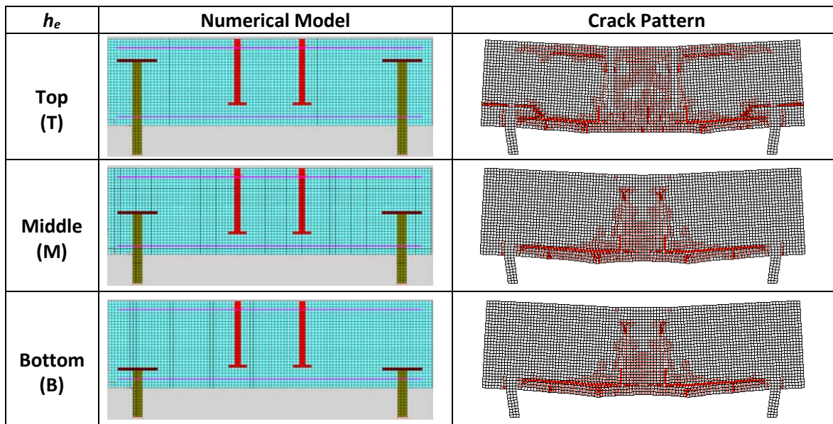
Figure A-19: Numerical model and crack pattern-single bracket type-monotonic compression - a/d ratio = 1.68, \rho_x = 0.2\% .
