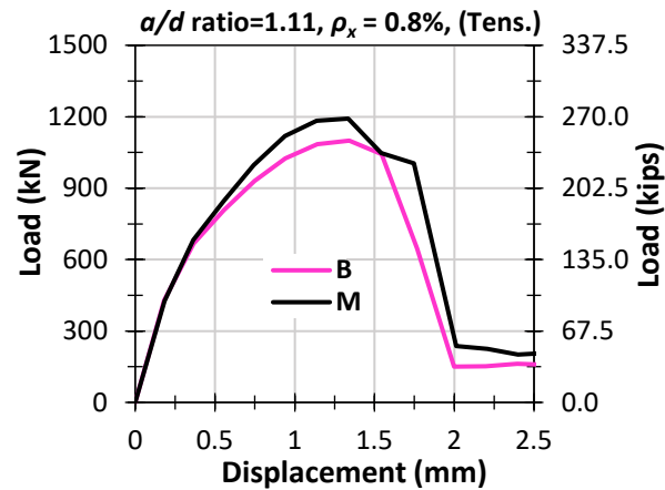
Figure C-18: Load-displacement response-studded bracket-monotonic compression- a/d=1.11 , \rho_x = 0.8\% .
