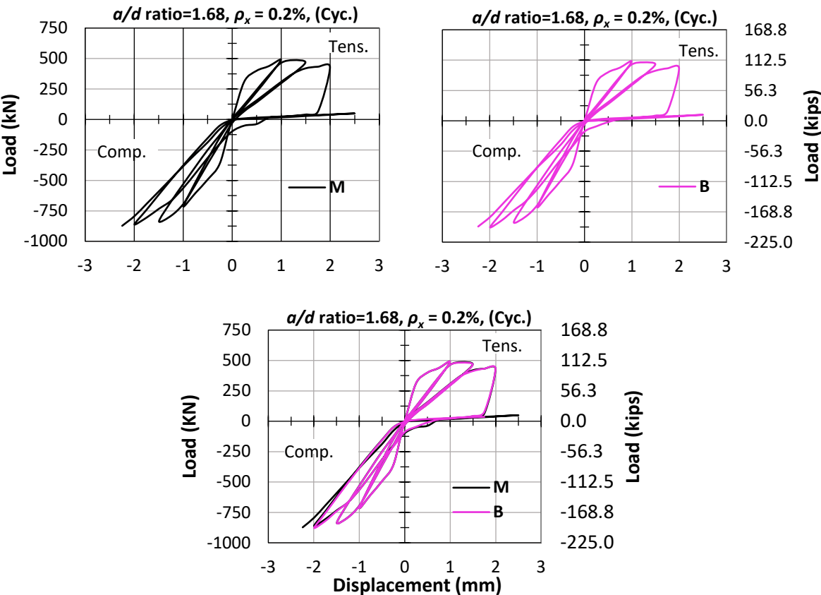
Figure C-38: Load-displacement response-studded bracket type-monotonic tension - a/d ratio = 1.68, \rho_x = 0.2\% .
