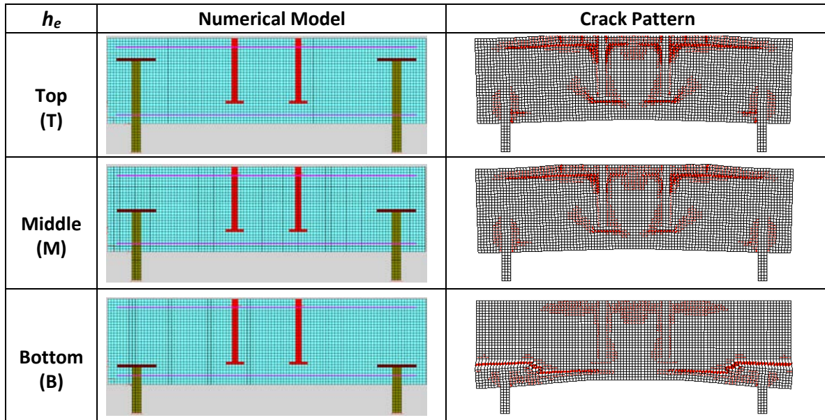
Figure A-3: Numerical model and crack pattern-single bracket type-monotonic tension - a/d ratio = 1.68, \rho_x = 0.4\% .
