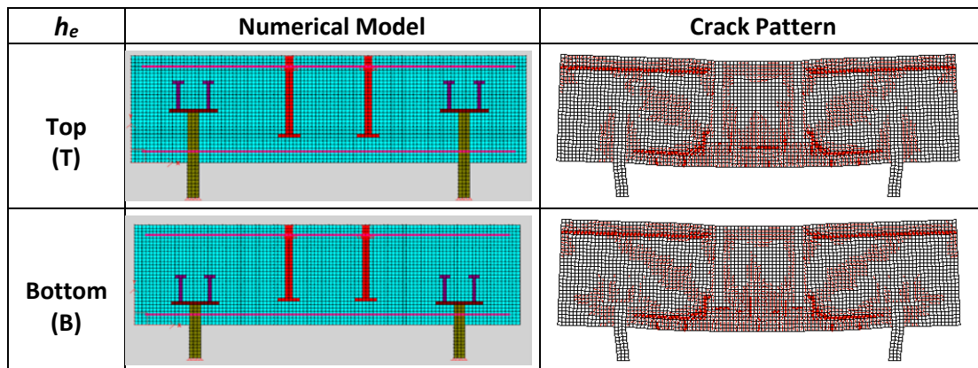
Figure C-45: Numerical model and crack pattern-studded bracket type-monotonic tension - a/d ratio = 1.42, \rho_x = 0.4\% .
