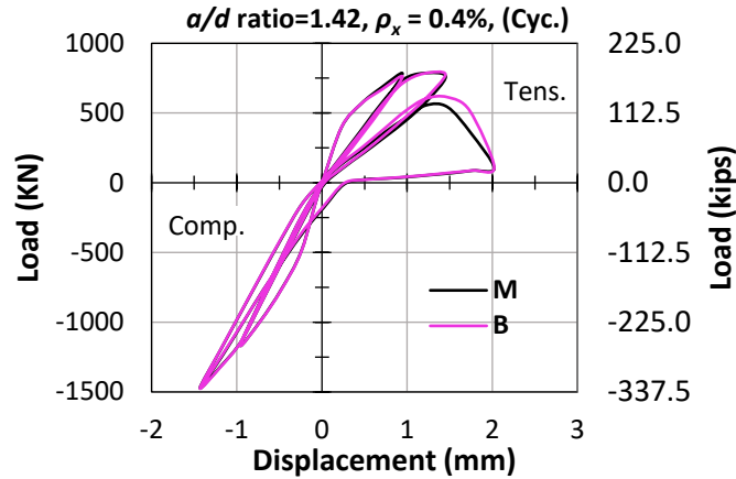
Figure C-46: Load-displacement response-studded bracket type-monotonic tension - a/d ratio = 1.42, \rho_x = 0.4\% .
