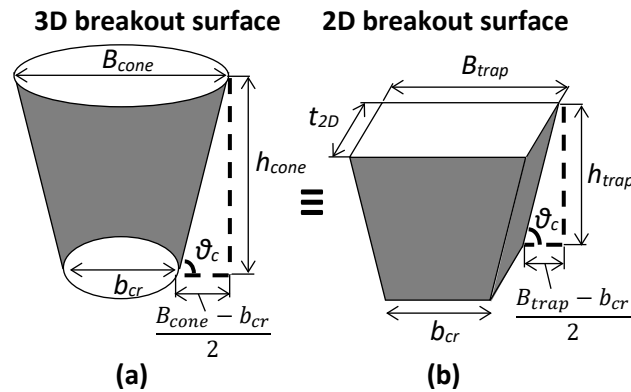
Figure 4-4: Surface area for (a) 3D; (b) 2D concrete breakout shapes.
