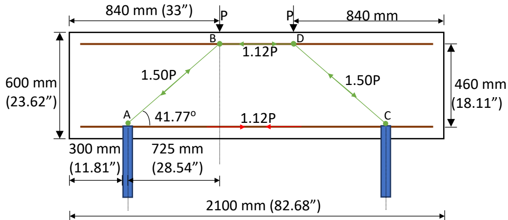
Figure D-3: Strut and Tie Model for one sample foundation.
